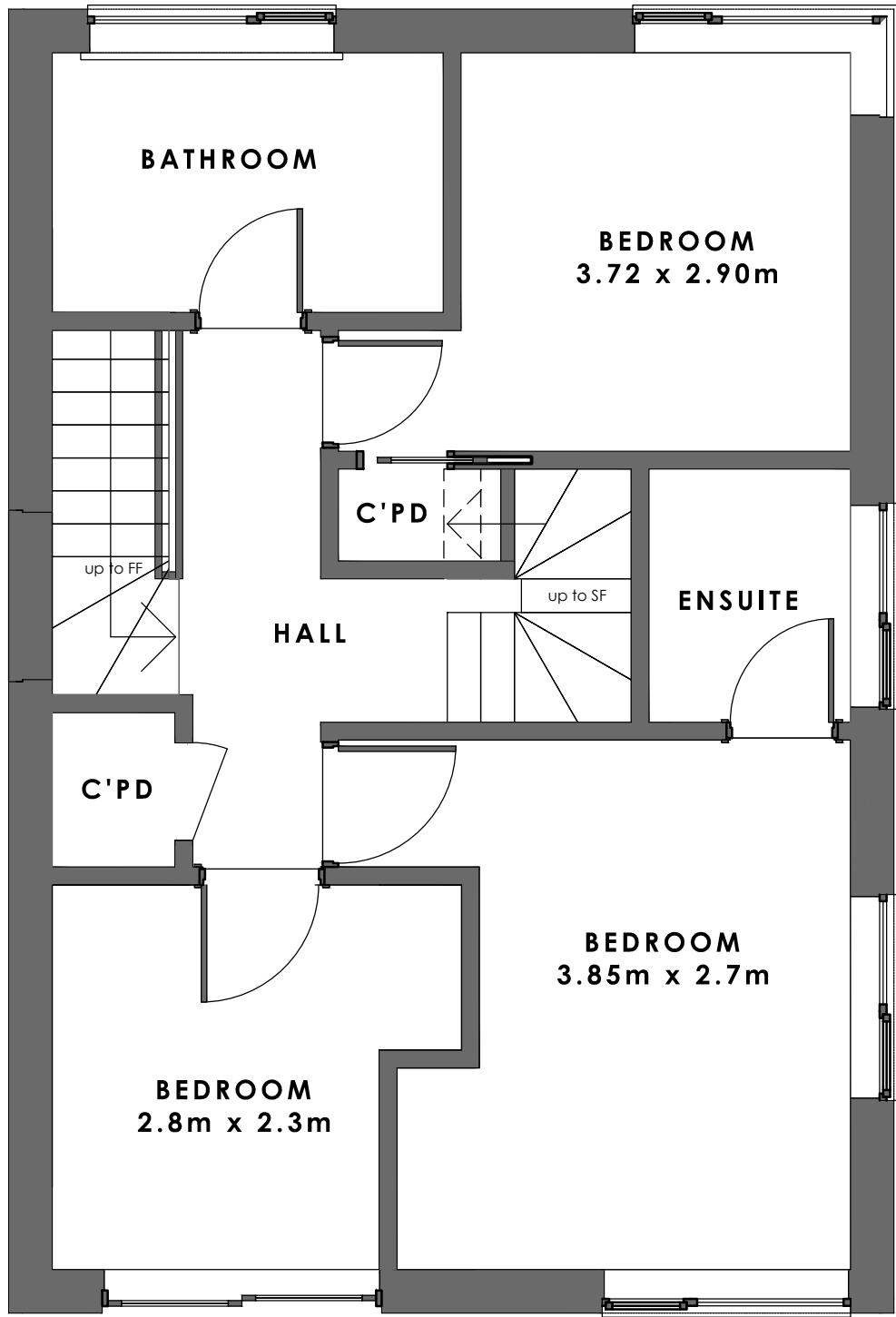
FIRST FLOOR PLAN APPROX FLOOR AREA 51.5 SQM
