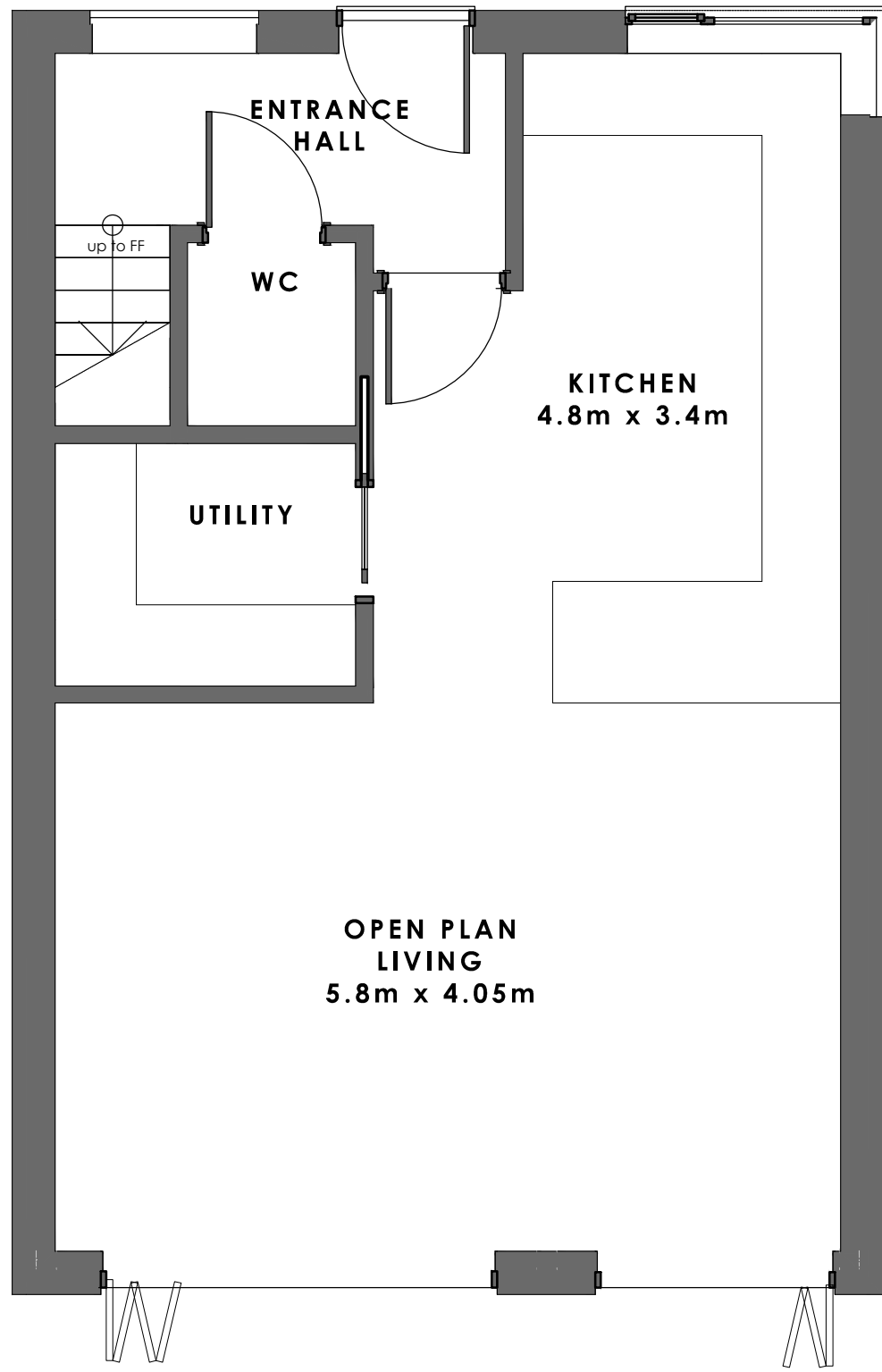
GROUND FLOOR PLAN APPROX FLOOR AREA 51.5 SQM
